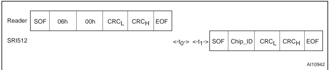
Figure 56. PCALL16 frame exchange between Reader and SRI512
